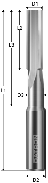
DATRON Reamers Standard Version
